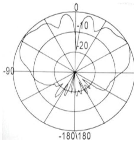
E Plane
